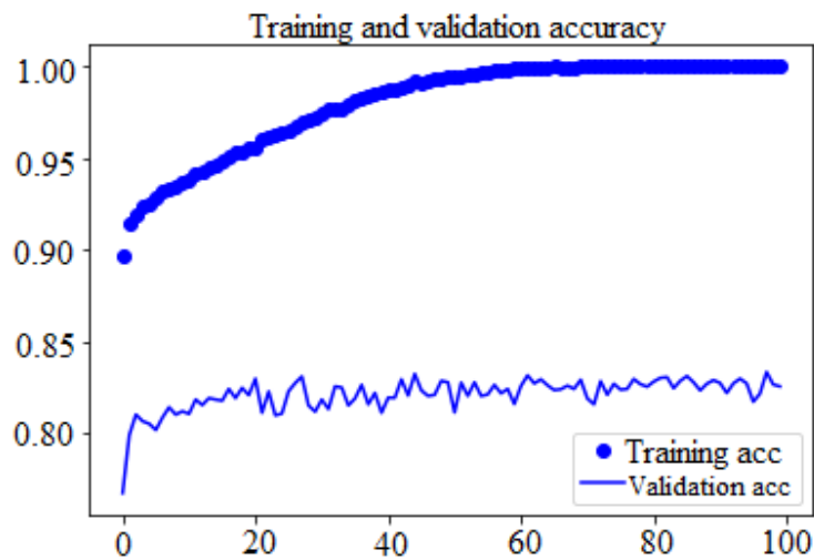
Figure 1. Training and validation accuracy of the VGG-19A model
