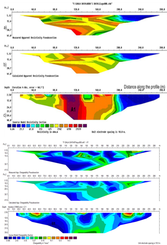
Figure 5. Resistivity and chargeability tomography of Profile 1
