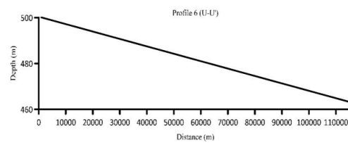
Figure 24. Profile 6 showing the cross-section U-U'
