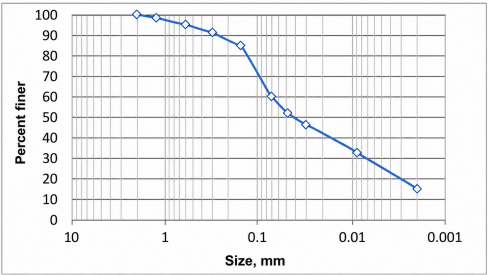
Figure 3. Grain size distribution curve of natural soil
