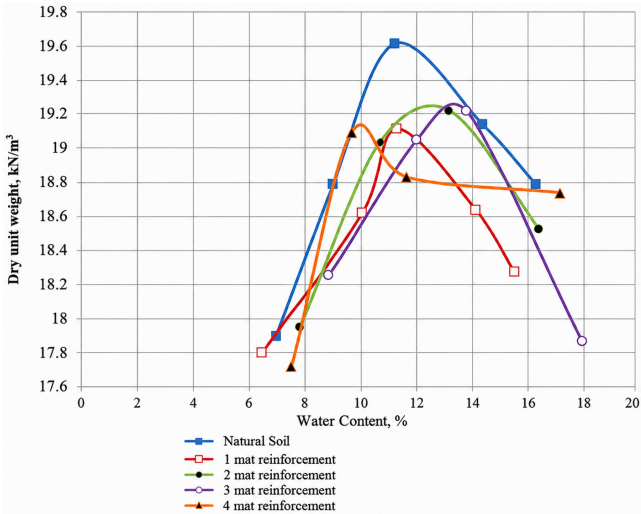
Figure 5. Compaction characteristics of soil with different mat reinforcement
