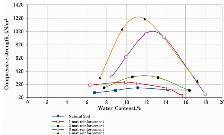
Figure 8. Strength characteristics of soil with different number of mat reinforcements
