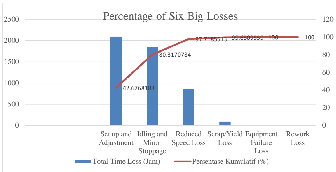
Figure 2: Pareto Diagram of Six Big Losses Percentage
