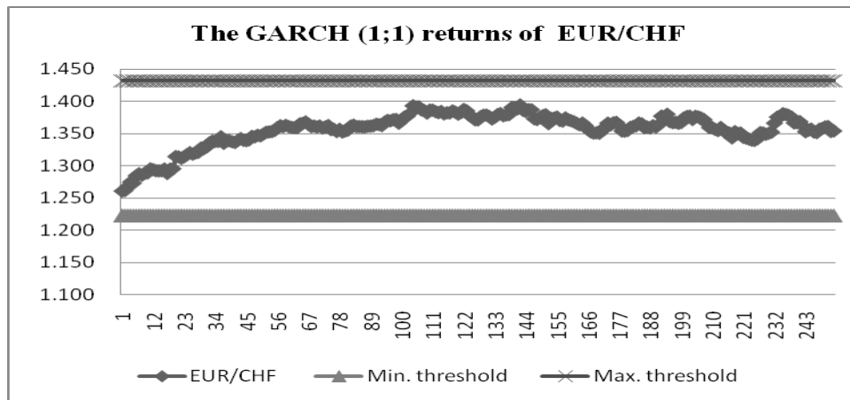
Figure 14: The EUR/CHF exchange rate return data estimated through GARCH (1;1)
