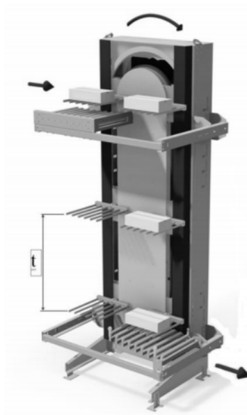
Figure 1. Paternoster chain conveyor with two heights
