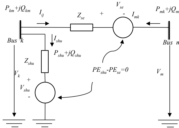
Figure 2. Equivalent circuit of UPFC
