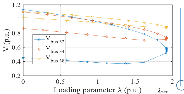
Figure 9. P-V curve for the 57-bus test system with UPFC
