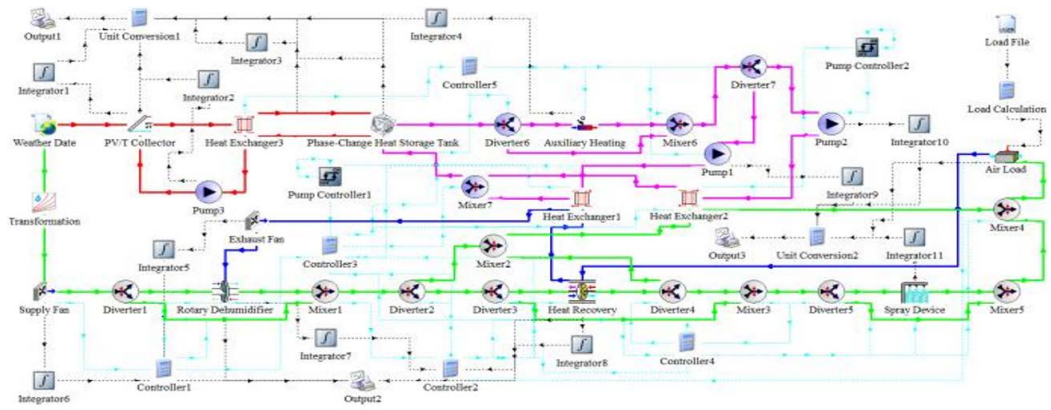
Figure 4. The model of new system based on TRNSYS18 Note: The red, green and blue solid lines represent water, supply and exhaust routes, respectively
