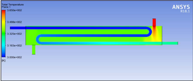
Figure 15. Temperature distribution with 4% nanofluid
