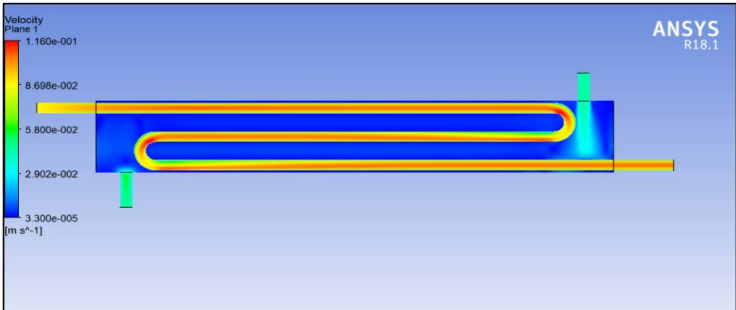
Figure 17. Velocity distribution with 4% nanofluid
