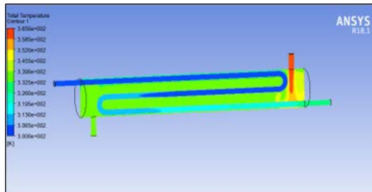
Figure 7. Temperature distribution with water as fluid
