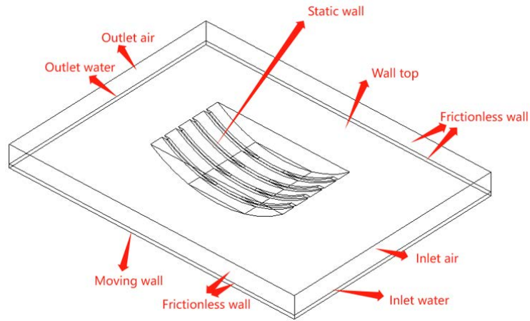
Figure 8. Boundary condition settings
