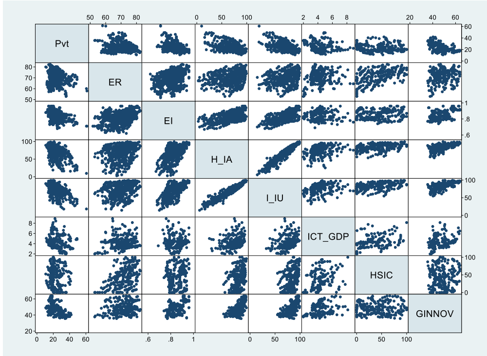
Figure 2. Scatterplot matrix of EU-27 indicators, 1995-2021 Source: Authors' contribution in Stata 17
