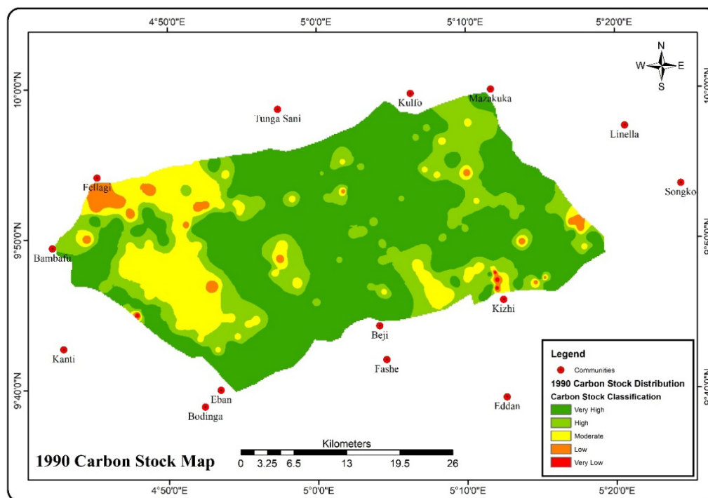
Figure 2. Spatio-temporal distribution of carbon stock in the Zuguuma sector (1990)
