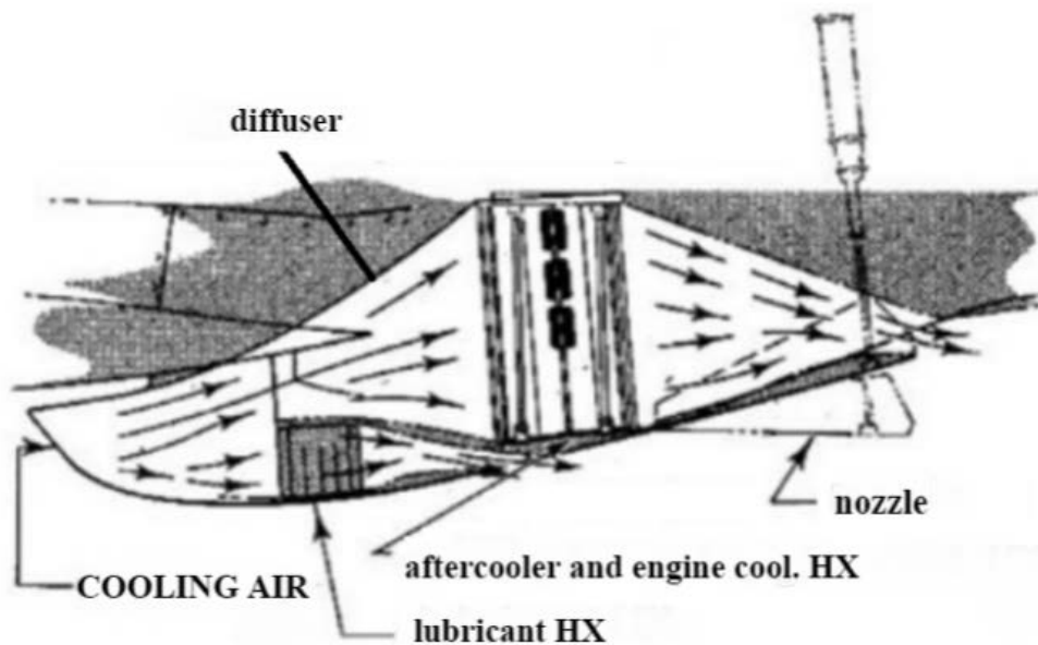
Figure 1. P51D cooling duct (rearranged from the flight manual)
