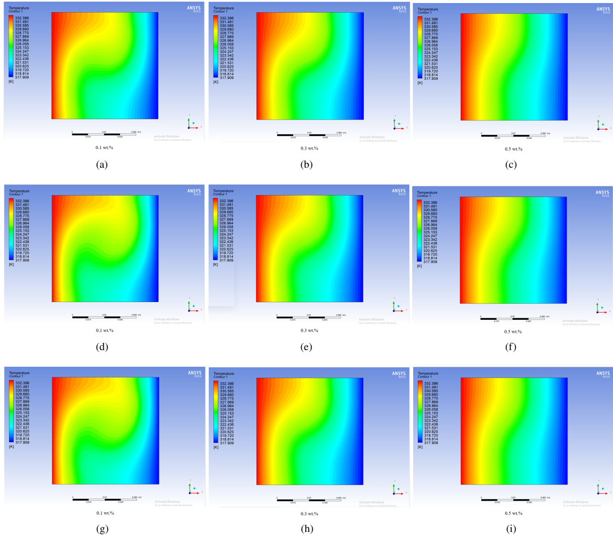
Figure 6. Temperature contours with 0.1, 0.3, and 0.5 wt.%, respectively (a-c) \text{Al}_2\text{O}_3 %; (d-f) \text{CuO} %; (g-i) \text{ZnO} %
