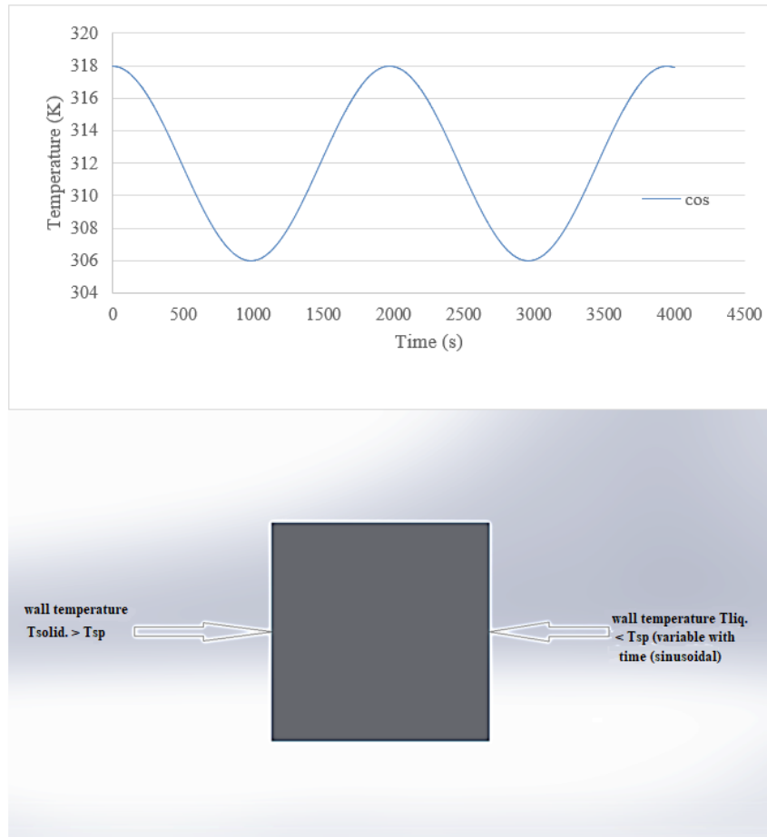
Figure 2. Gradually varying temperature over time as a Cos profile
