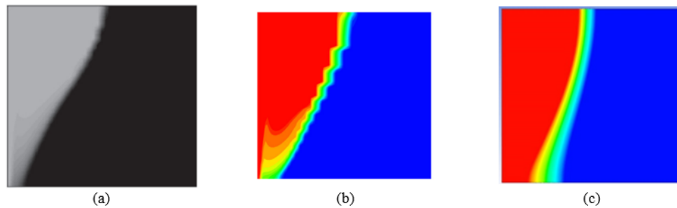
Figure 3. Validation of (a, b) previous studies and (c) this study
