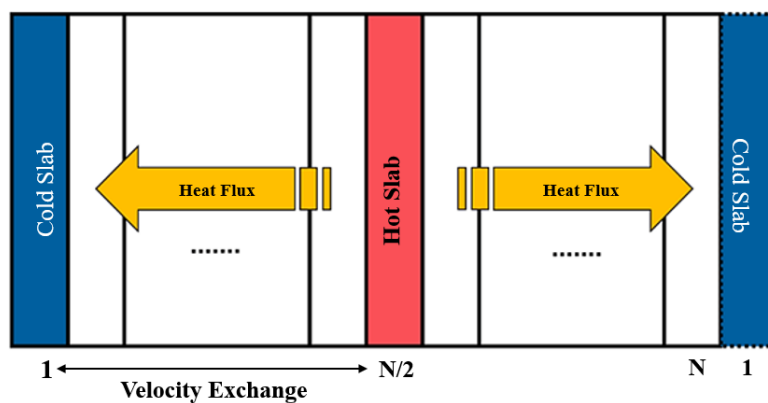
Figure 2. Thermal conductivity measurement using NEMD [16]
